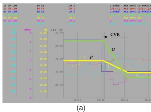
Figure 32: Active power reduction on HV/MV transformer level by changing-over the ZUQDE functionality. a) real time recording; b) active power reduction for different loading cases.
